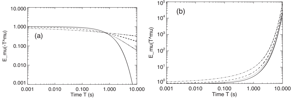
Figure 3: The feature of the Mittag-Leffler function (a) E_\mu(-T^\mu) and (b) E_\mu(T^\mu) as a function of time T . Solid line \mu = 1 , dotted line \mu = 0.75 , dashed line \mu = 0.50 and dash-dot line \mu = 0.25 .
