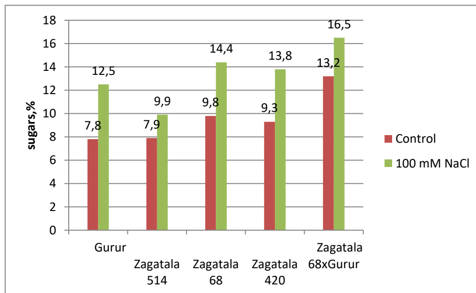
Fig. Influence of sodium chloride on content sugars in seedlings of maize varieties
