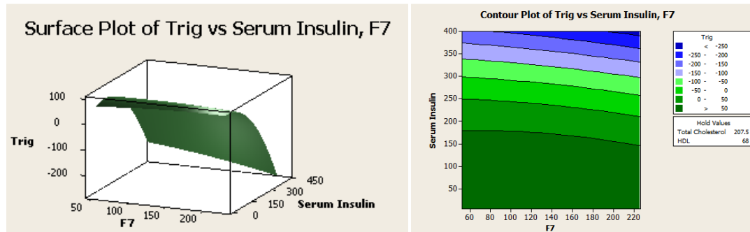
Figure 9. Surface Plot for Triglycerides vs Serum Insulin, Proconventin (F7)
