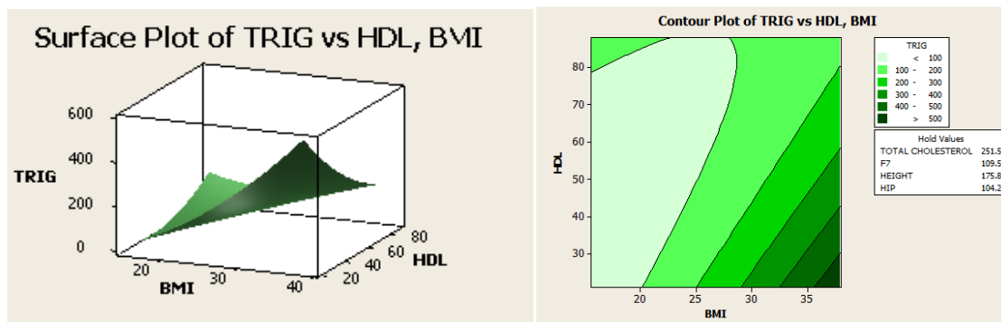
Figure 3. Surface Plot for Triglycerides vs High Density Lipoprotein, Body Mass Index
