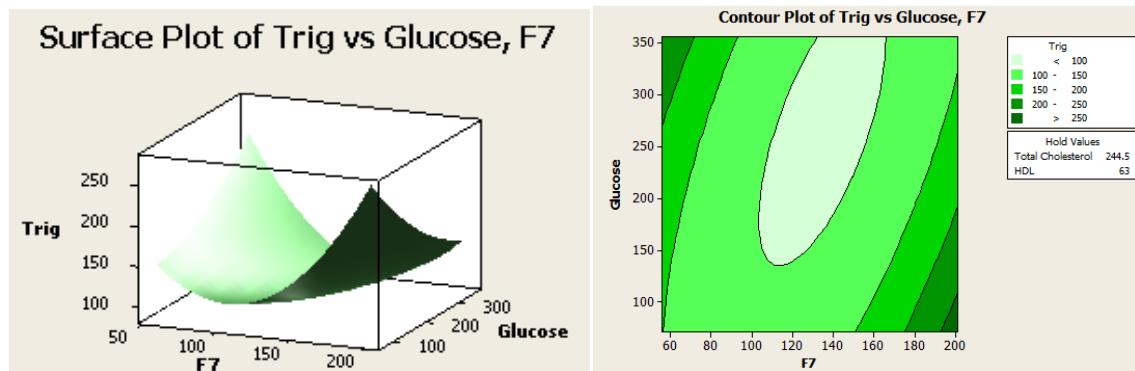
Figure 5. Surface Plot for Triglycerides vs Glucose, Proconventin (F7)
