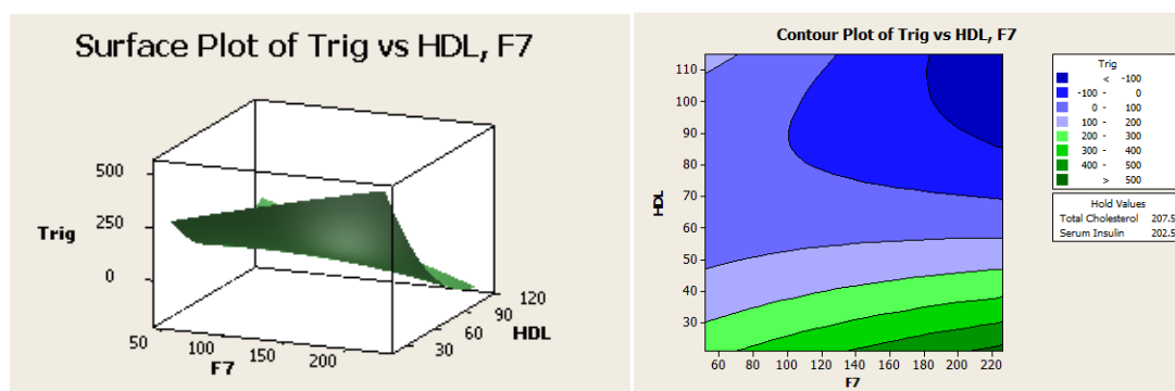
Figure 8. Surface Plot for Triglycerides vs High Density Lipoprotein, Proconvertin (F7)
