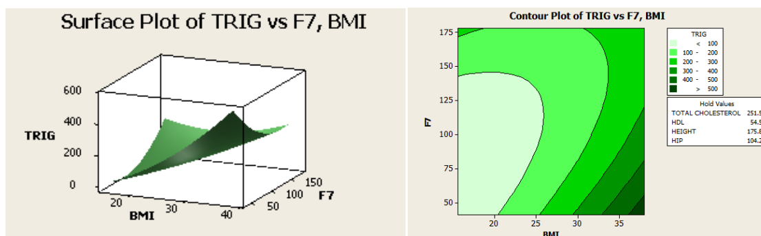
Figure 1. Surface Plot for Triglycerides vs Proconvertin (F7), Body Mass Index
