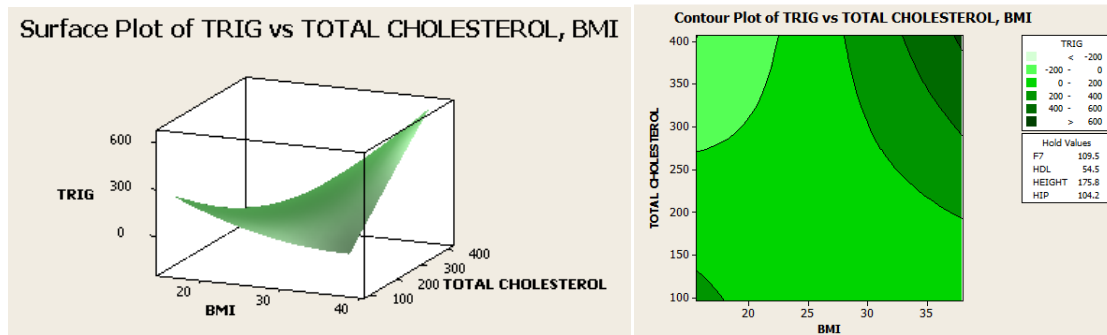
Figure 2. Surface Plot for Triglycerides vs Cholesterol, Body Mass Index
