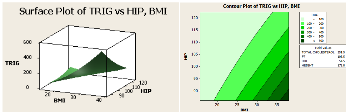
Figure 4. Surface Plot for Triglycerides vs Hip Circumference, Body Mass Index
