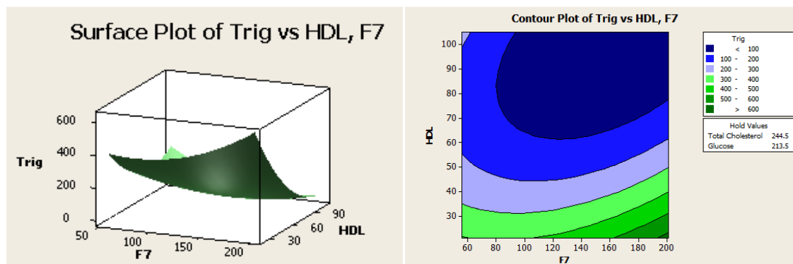
Figure 6. Surface Plot for Triglycerides vs High Density Lipoprotein, Proconventin (F7)
