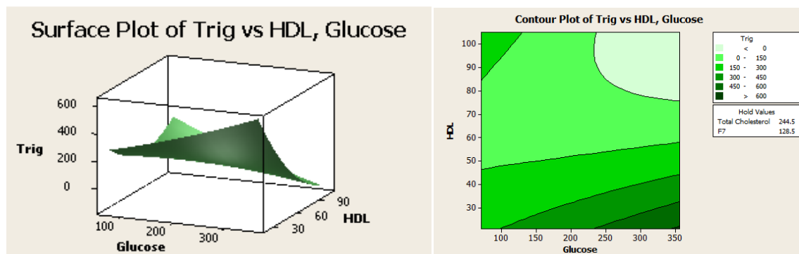
Figure 7. Surface Plot for Triglycerides vs High Density Lipoprotein, Glucose
